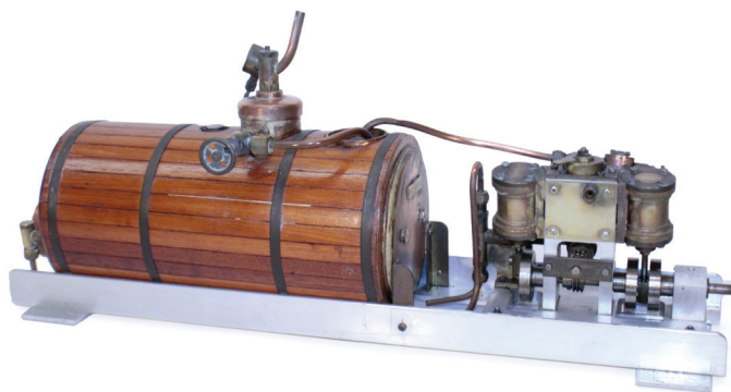
Featured item: Lot 159 Live Steam 2-cylinder Marine Engine
